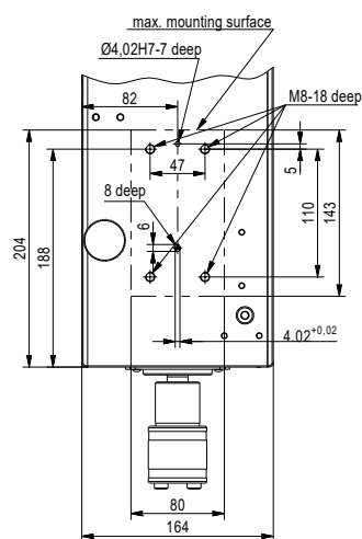
Fig.: Flange dimensions of the drive unit Taurox 900E
