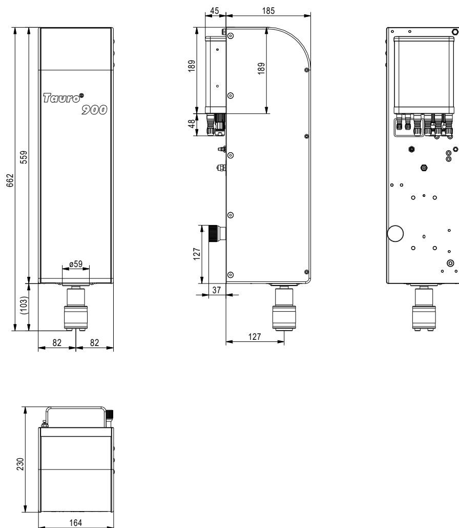
Fig.: View of the thread drive unit Taurox 900E
