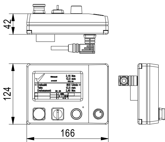
Fig.: View of the operating panel Taurox 900E
