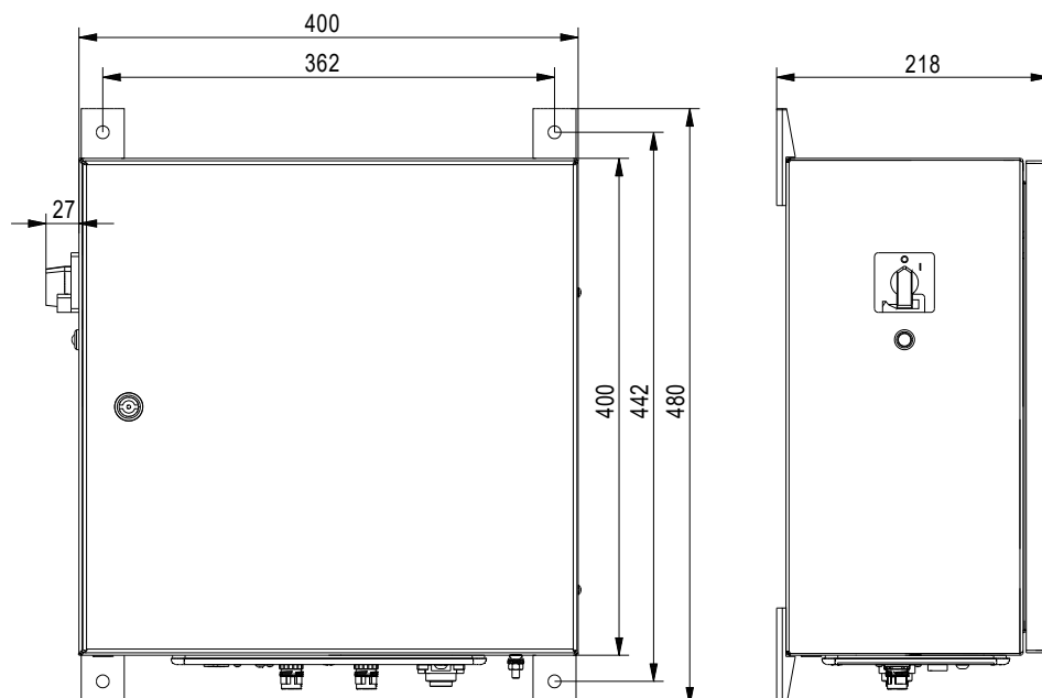
Fig.: View of the control unit Taurox 900E
