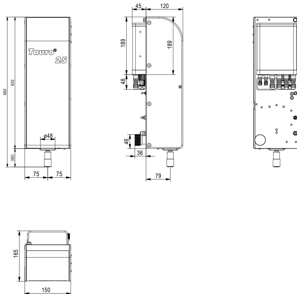
Fig.: View of the thread drive unit Tauro 25E
