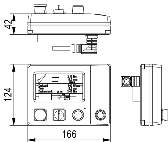
Fig.: View of the operating panel Tauro 25E
