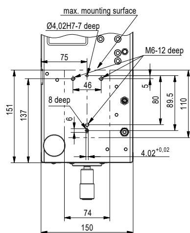
Fig.: Flange dimensions of the drive unit Tauro 25E
