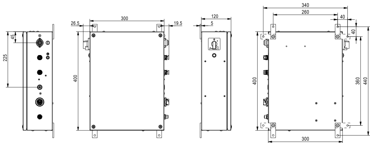
Fig.: View of the control unit Tauro 25E with fixation to wall
